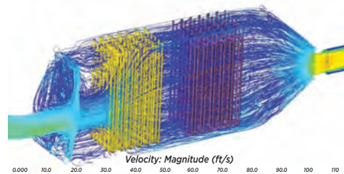
CFD of heater box
