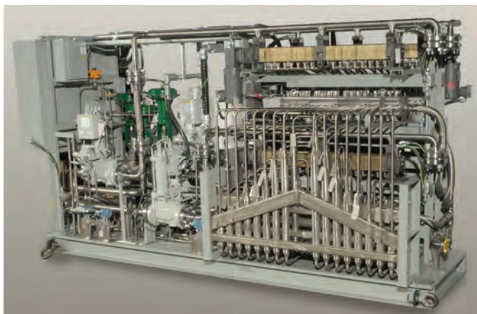
Fuel oil/water injection system
